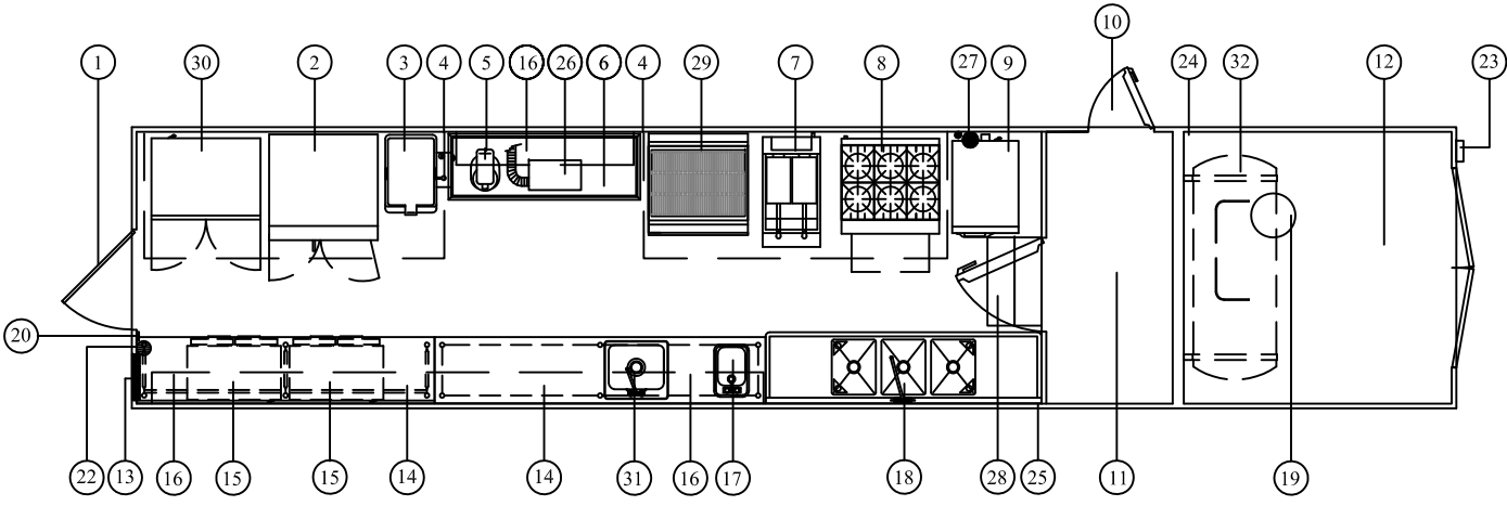
Floor Plan
